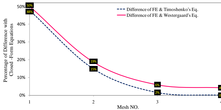
Figure 2 FE elastic analysis, compared with closed-form solutions
